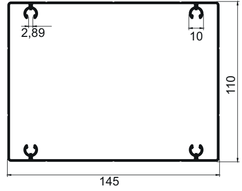
P-107 Ayak 100x145 3,440 kg/m
