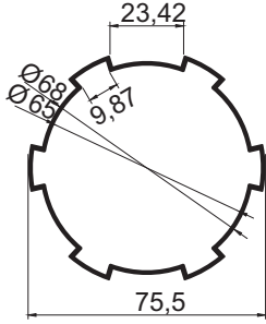
P-105 75'lik Boru 1,100 kg/m
