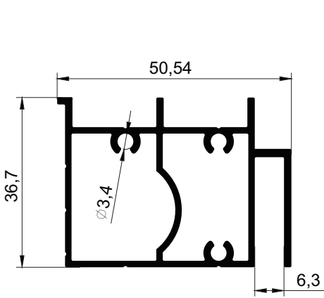
RK-501 DİKEY BAZA 0.946 kg/m
