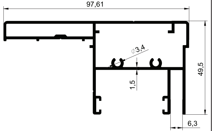
RK-502 SABİT DİKME 1.526 kg/m
