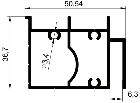
RK-501 DİKEY BAZA 0.946 kg/m
