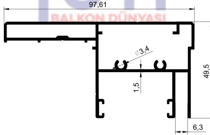
RK-502 SABİT DİKME 1.526 kg/m
